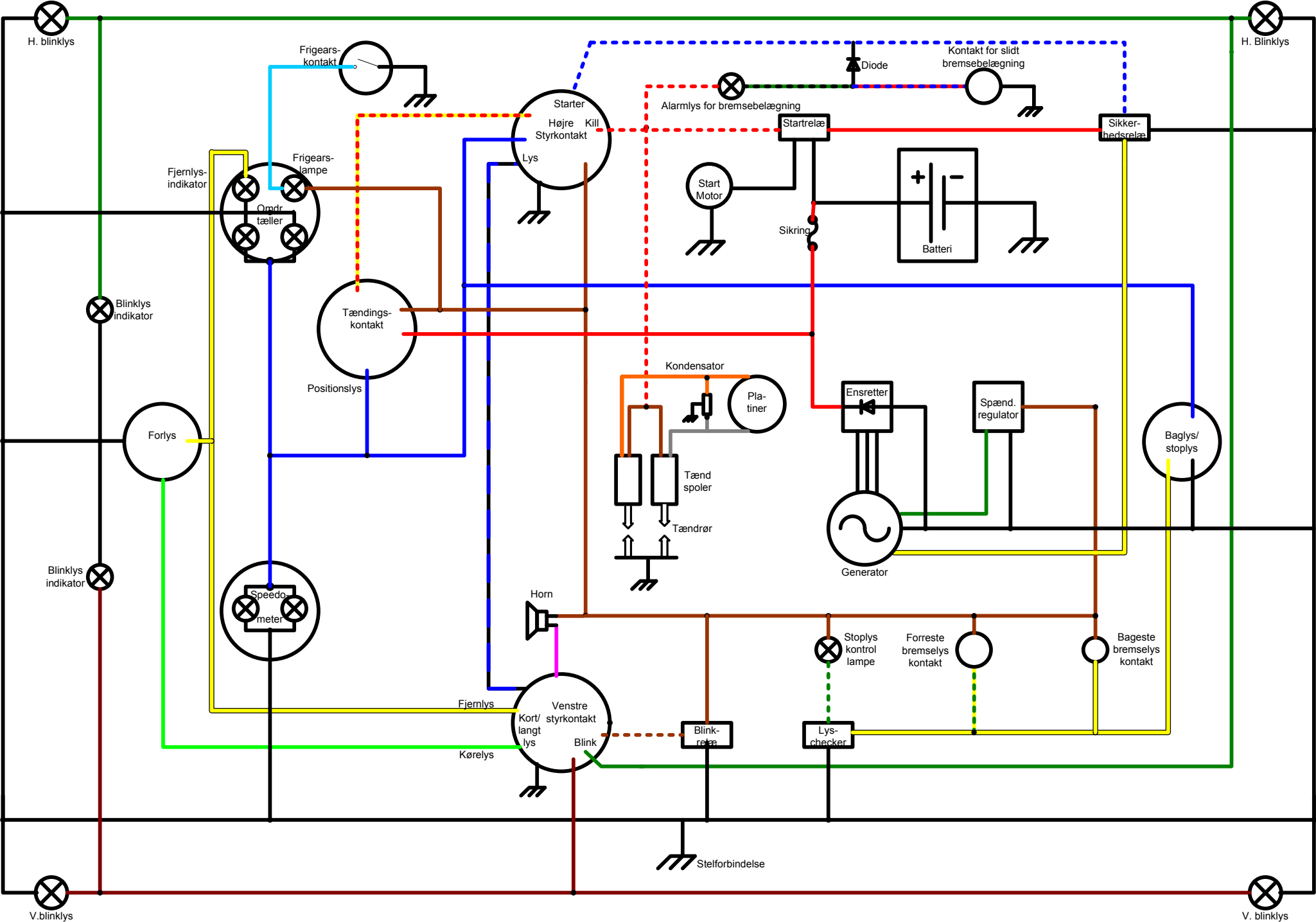
Eldiagram TX650A, XS650B & XS650C
